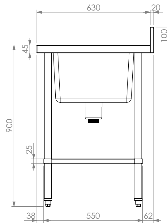
SIDE ELEVATION
